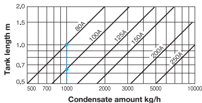
Chart 3 Sizing chart of closed receiver
