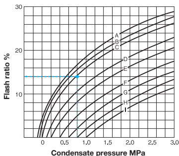
Chart 1 Flash rate of Condensate
